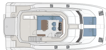
SKYLounge FLYBRIDGE W/ INTERIOR STAIRS & CAPTAIN CHAIRS
