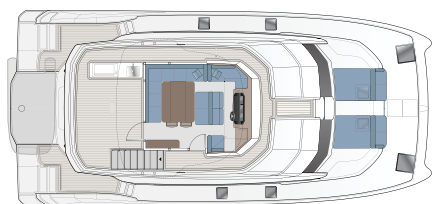
SKYLounge FLYBRIDGE W/ NO INTERIOR STAIRS & STANDARD SEATING
