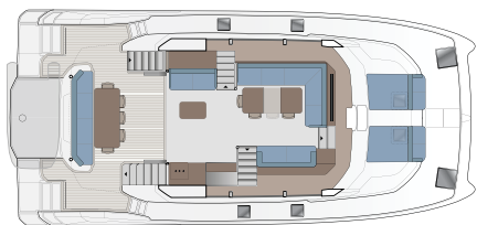
MAIN DECK W/GALLEY DOWN
