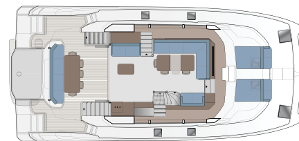
MAIN DECK W/GALLEY DOWN INTERIOR SKYLounge FLYBRIDGE STAIRS
