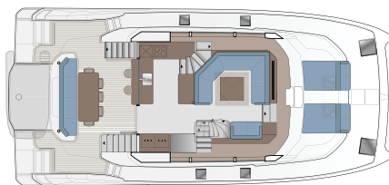
MAIN DECK W/INTERIOR SKYLounge FLYBRIDGE STAIRS W/SKYLounge
