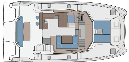
OPTIONAL MAIN DECK W/ INTERIOR HELM
