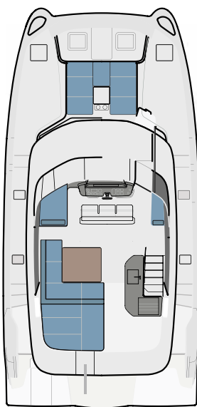
STANDARD FLYBRIDGE
