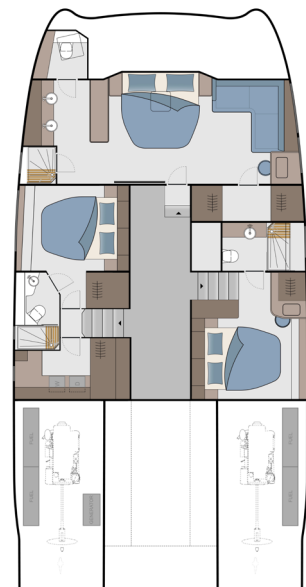
STANDARD 3-CABIN, +UTILITY ROOM
