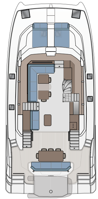
MAIN DECK GALLEY DOWN (SKYLounge FLYBRIDGE)
